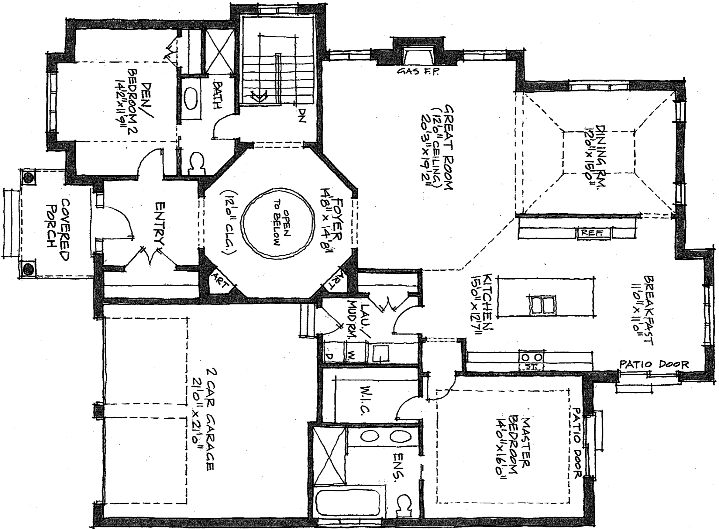
MAIN FLOOR PLAN - 2215 SQ. FT. + 20 SQ. FT. OPEN
