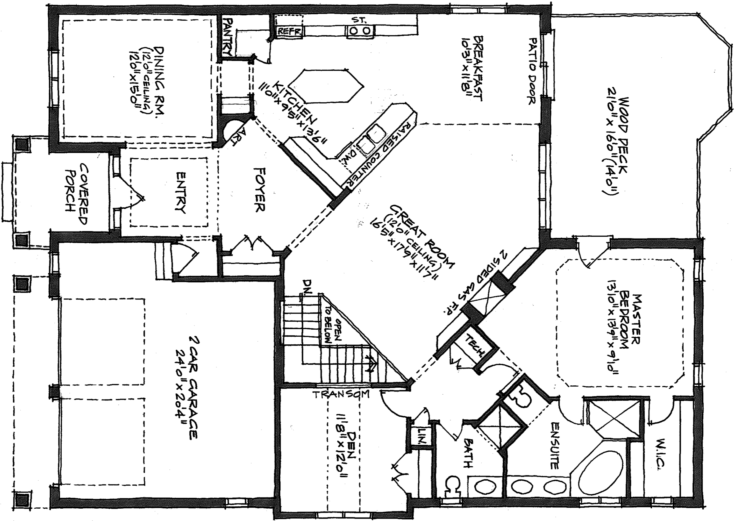
MAIN FLOOR PLAN - 2016 SQ. FT. + 34 SQ. FT. OPEN
